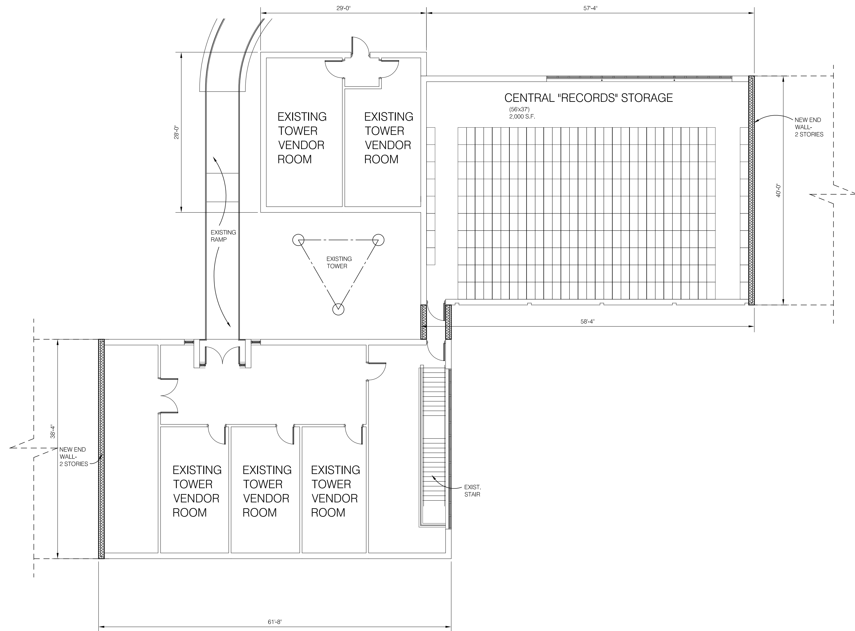
PORTION OF EXISTING COMM-DPW BUILDING TO REMAIN - UPPERLEVEL SCALE: 1/8" = 1'-0"
