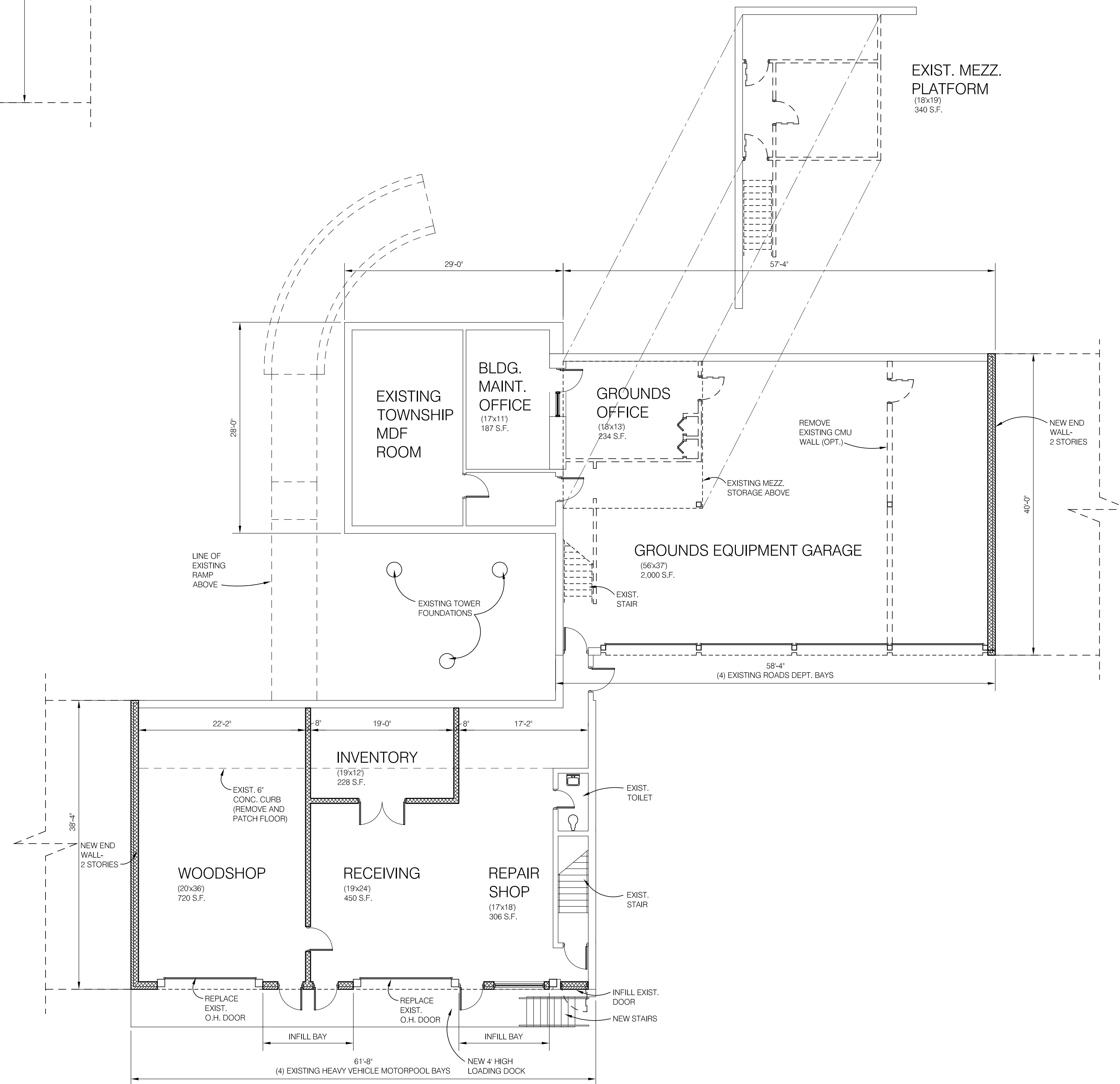
PORTION OF EXISTING COMM-DPW BUILDING TO REMAIN - LOWER LEVEL SCALE: 1/8" = 1'-0"
